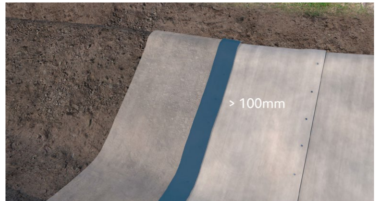
Overlap CC layers by a minimum of 100mm
