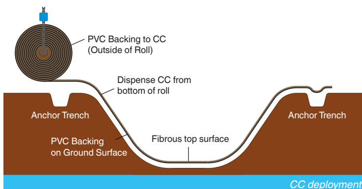
Substrate preparation & anchor trench
