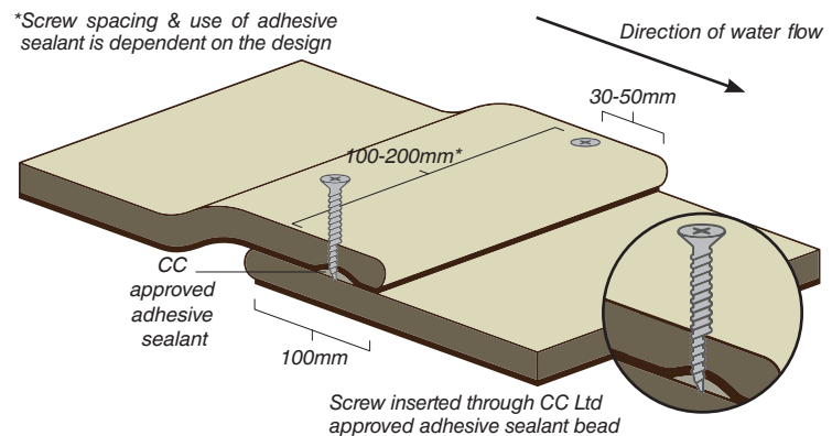
Typical screwed/screwed and sealed overlap joint
